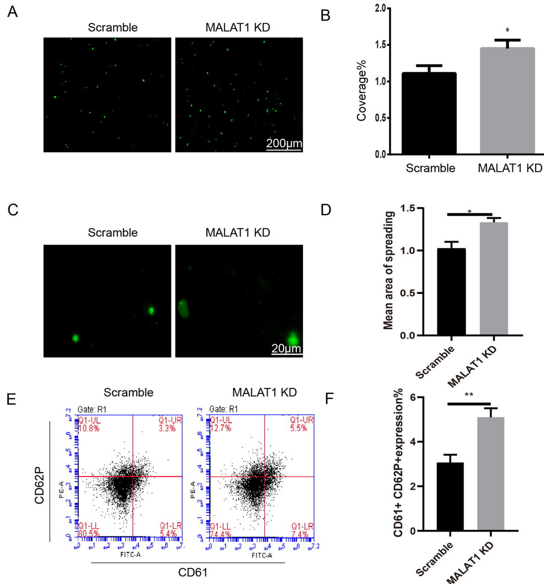
Figure 3 MALAT1 represses PLP adhesion, spreading and activity. (A) Adhesion of PLPs (green) from MALAT1 KD and control CD34 + megakaryocytes after treatment by thrombin 1 U/mL (scale bar, 200 μm). Three separate sets of data were collected for each experiment. (B) A statistical examination of the adhesion area of PLPs in coverslips that were coated with collagen. The values are shown as the mean±SD (*p<0.05). (C) A comparison of the capacity of PLPs to spread derived from MALAT1 kD CD34 + megakaryocytes and the scramble in the presence of thrombin at a concentration of 1 U/mL on coverslips coated with collagen (scale bar, 20 μm). (D) Histogram showing the relative area of PLPs for MALAT1 KD and scramble. Data are from three independent experiments. Error bars denote SD *p<0.05. (E) Flow cytometric analysis of CD61 and CD62P expressions on the PLPs isolated from MALAT1 kD megakaryocytes and scramble. (F) Histogram showing the proportions of CD61 + CD62P + cells for MALAT1 kD megakaryocytes and scramble group. Data are from three independent experiments. Error bars denote SD **p<0.01. KD, knockdown; PLPs, platelet-like particles.
