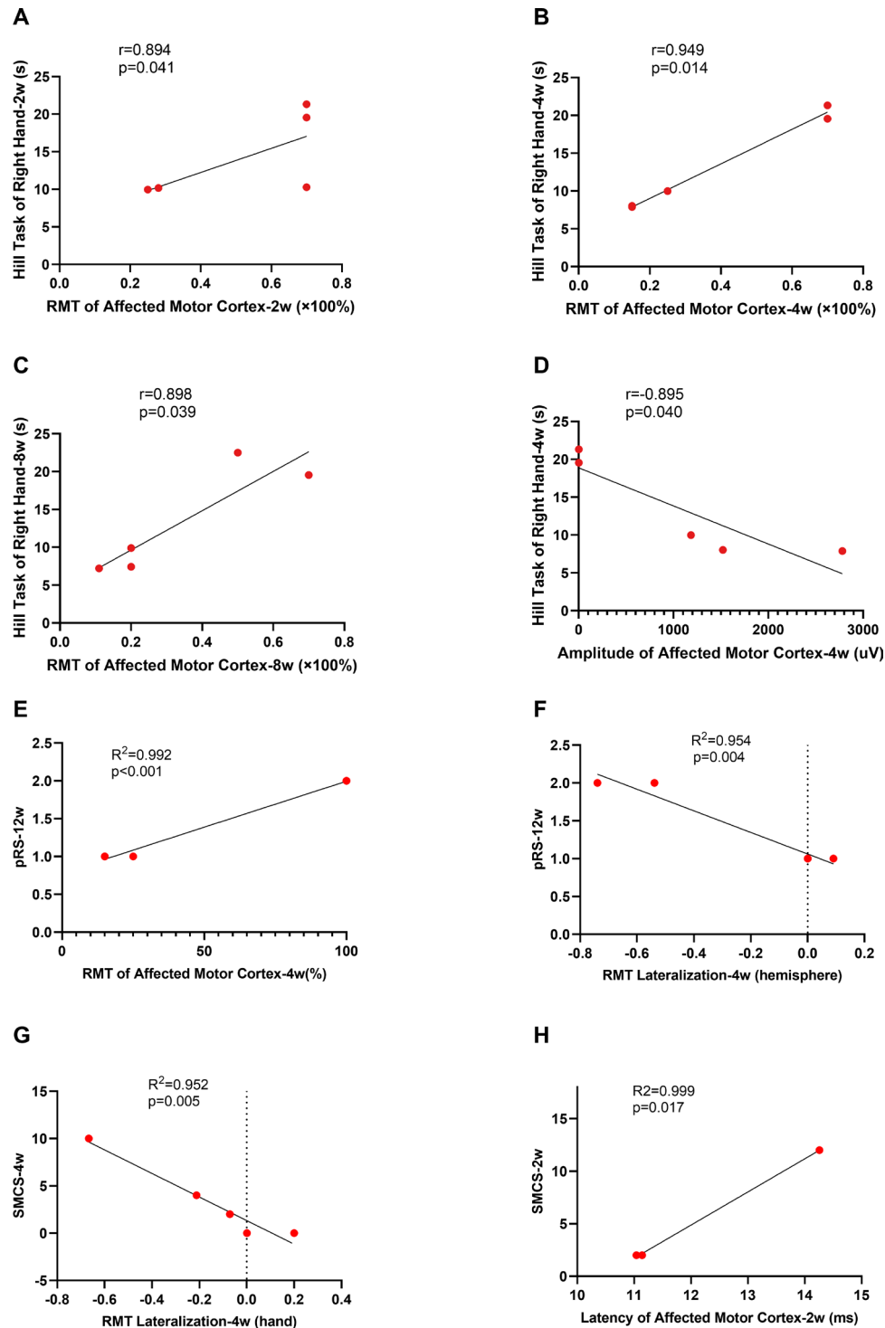
Figure 8 Correlation analysis.
